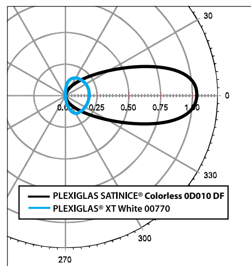
Figure 4: Polar diagram of luminance as a function of angle
