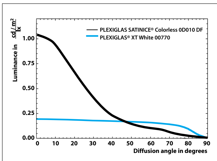
Figure 3: Diffusion indicatrix of luminance as a function of angle
